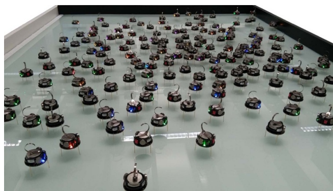
Figure 31. A swarm of Kilobots, a de facto standard platform for swarm robotics research. This is a small robot of 3.3 cm diameter, designed to move on a flat surface and communicate efficiently with its immediate neighbours. Several design choices have been made to simplify the electromechanical components and experimental procedures like recharging and uploading control programs—which become cumbersome with large swarms—enabling experimentation with thousand robots lasting several hours [165].
