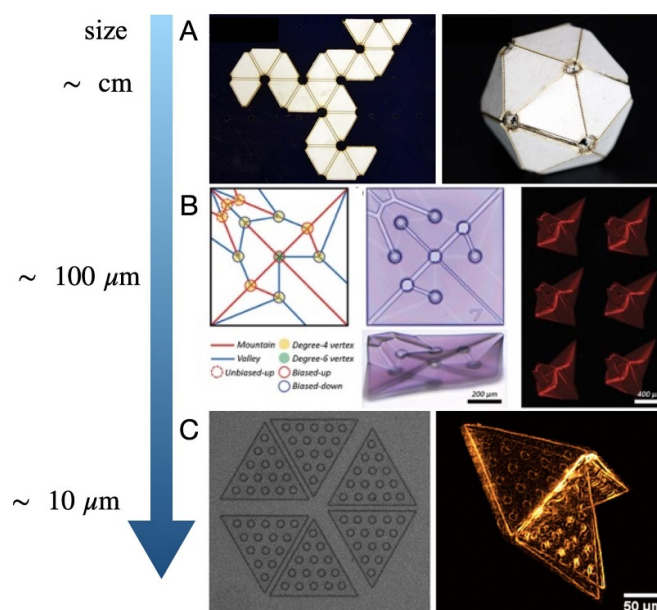
Figure 17. Self-folding orikata spanning multiple scales. (A) Macroscopic shape memory composite by heating. Reproduced from [103]. © IOP Publishing Ltd. All rights reserved. (B) Polymer trilayer folded by swelling. [110] John Wiley & Sons. © 2019 WILEY-VCH Verlag GmbH & Co. KGaA, Weinheim. (C) Folding nanofilms. Reprinted with permission from [104]. Copyright (2020) American Chemical Society.
