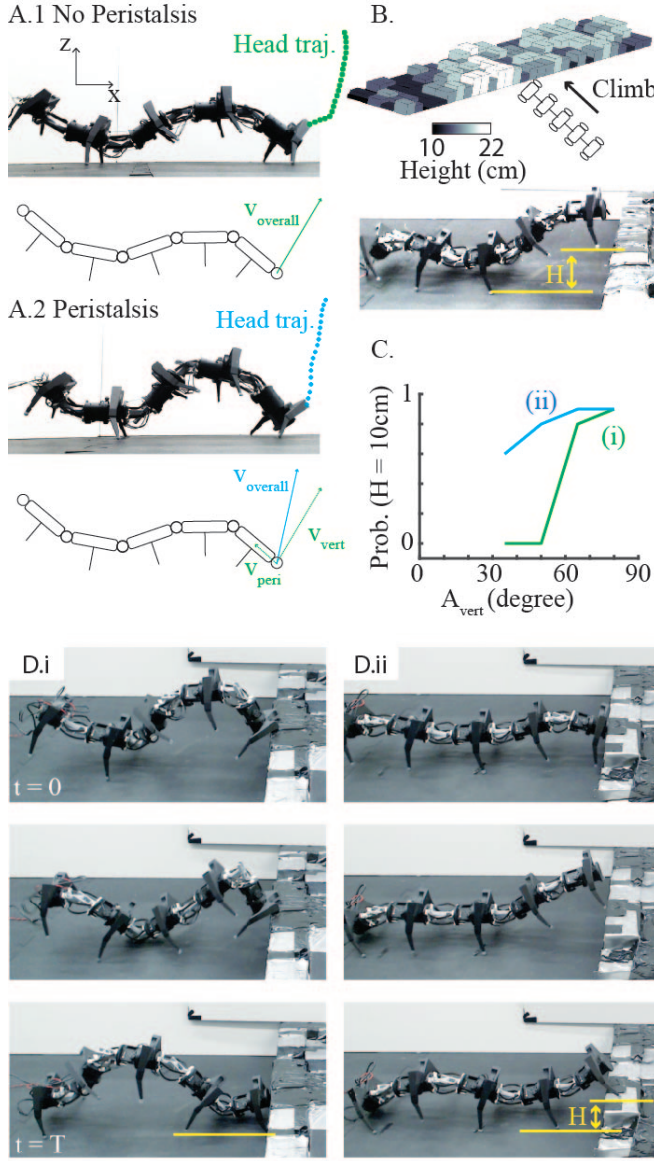
Fig. 6. Peristalsis wave to improve obstacle-climbing capabilities. (A.1) (top) Snapshot of pitch-only robot version at A_{vert} = 80^\circ and \Delta l = 0\text{cm} . Head movement trajectory is presented in green dots (obtained from experiments). (bottom) A diagram illustrating the head velocity components for pitch-only robot locomotion. (A.2) Snapshot of two-DoF robot version at A_{vert} = 80^\circ and \Delta l = 1\text{cm} . Head movement trajectory is presented in blue dots (obtained from experiments). (bottom) A diagram illustrating the head velocity components for two-DoF robot locomotion. (B) (top) A diagram illustrating the rugose terrain. The terrain has an average height difference of about 0.6 times robot's height. (bottom) The edge of the terrain is 10-15 cm from the ground, comparable to the robot's height. (C) Probability of climbing over obstacles for robot (blue, \Delta l = 1\text{cm} ) using a peristaltic wave and (green, \Delta l = 0\text{cm} ) not using a peristaltic wave, both as a function of A_{vert} . (D) Snapshot of (i) A_{vert} = 80^\circ and \Delta l = 0\text{cm} (without peristalsis) failing to climb up the step and (ii) A_{vert} = 35^\circ and \Delta l = 1\text{cm} (with peristalsis) succeeding to climb the step. Full videos can be found in SI.
