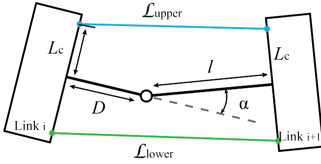
Fig. 2. Geometry of an individual joint. L_{upper} and L_{lower} refer to the length of the upper and lower cables. D and L_c are dimensional constants of the robot. l and \alpha are the peristaltic length and the joint angle controlled by the gait equation, respectively.
